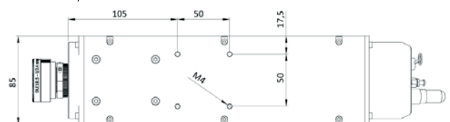
Cased camera, bottom view
