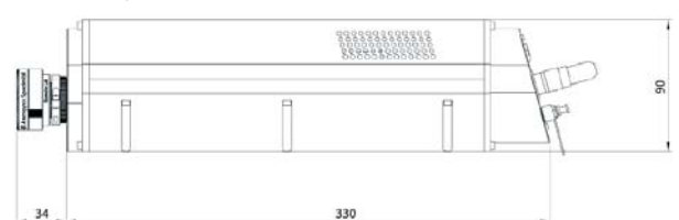
Cased camera, side view
