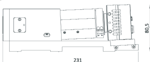
OEM camera, side view
